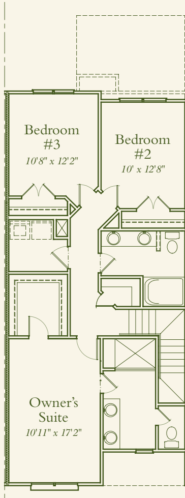
SECOND FLOOR
